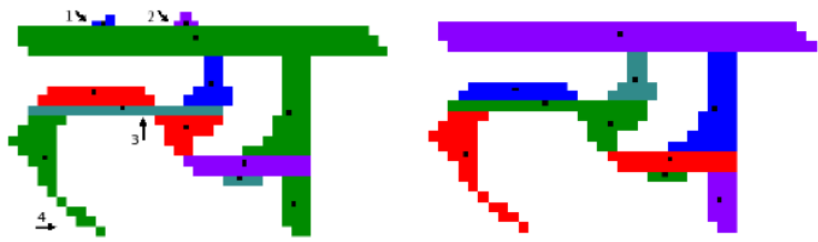
Fig. 5. Illustration of BAG-based noise removal – Left: (1, 2) sample with noise (3) thin joint (4) thin ligature boundary, Right: result of BAG-based noise removal [10]
